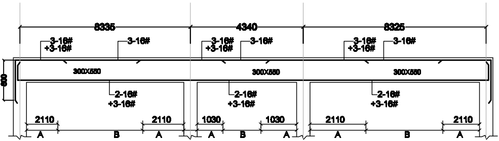
RB.BEAM-A1,B1,C1,D1/A4,B4,C4,D4 BEAM SIZE- 300X550
