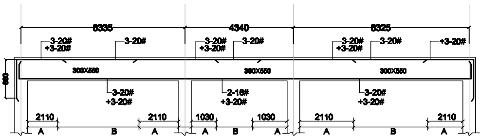
RB.BEAM-A2,B2,C2,D2,/A3,B3,C3,D3, BEAM SIZE- 300X550
