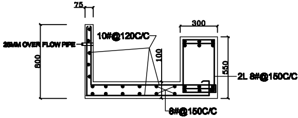
DETAIL OF GUTTER
