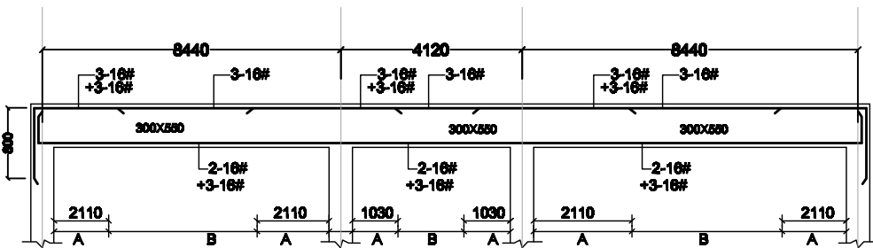
RB.BEAM-A1,A2,A3,A4/B1,B2,B3,B4 C1,C2,C3,C4/D1,D2,D3,D4 BEAM SIZE- 300X550
